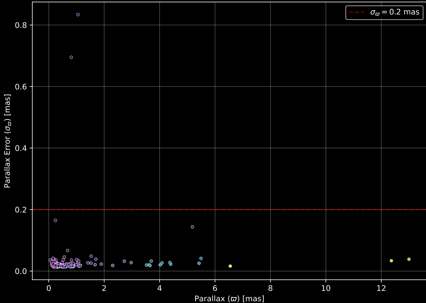
APOGEE DR17 Field: [214+04] Parallax Quality (n= 179)
