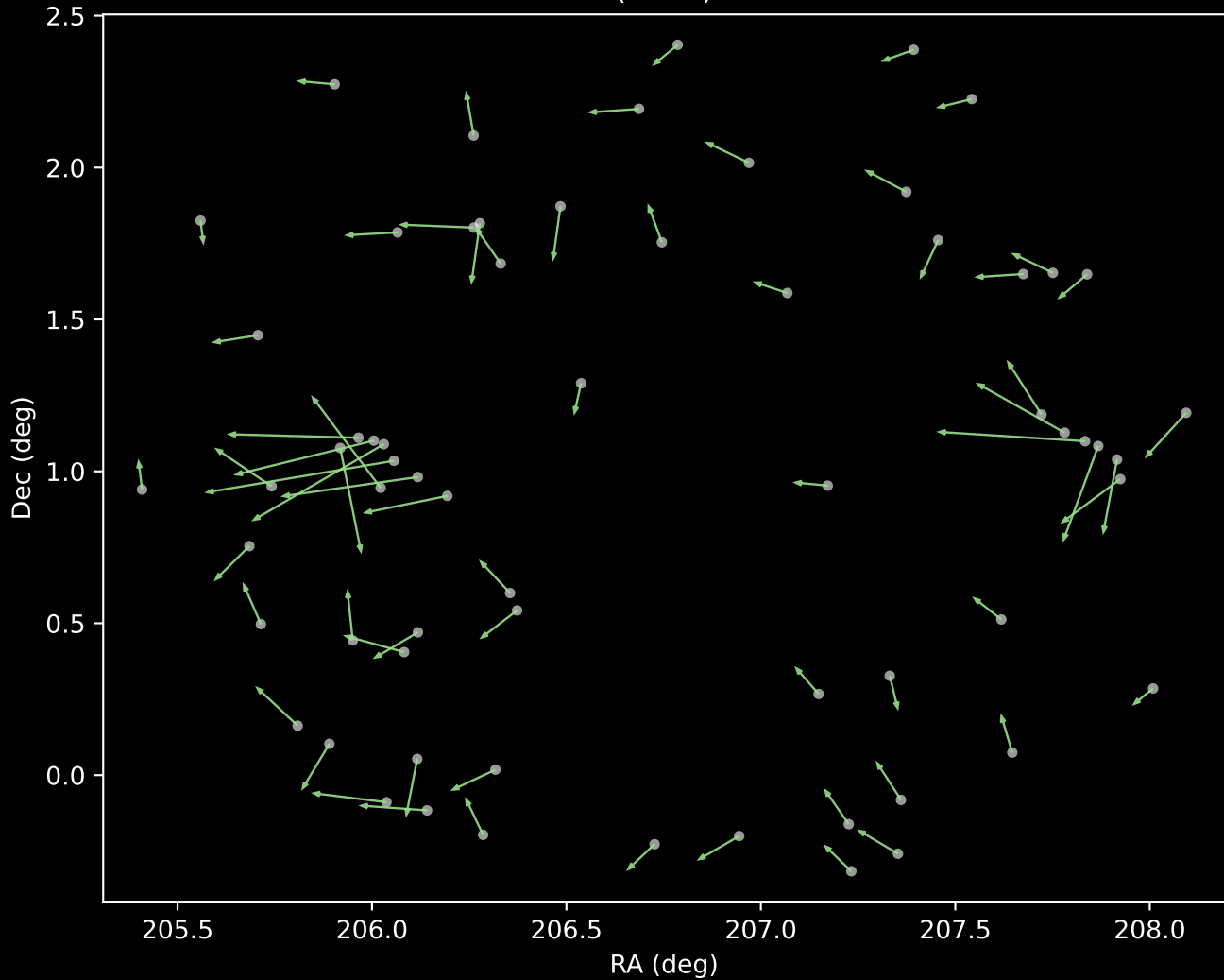
APOGEE DR17 Cluster 5 Proper Motion Vectors (n=65)
