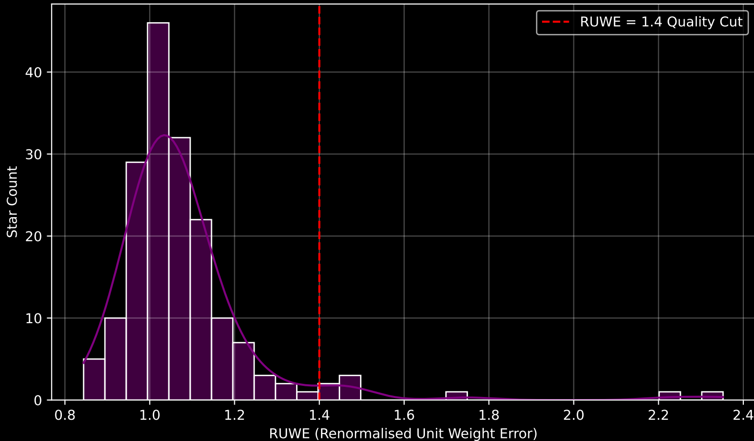
GAPOGEE DR17 Field [214+04] RUWE Distribution (n= 175)
