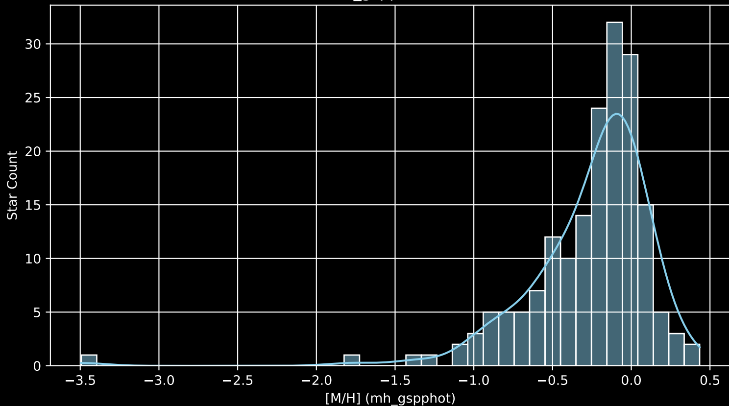
APOGEE DR17 Field: [214+04 [M/H] (mh_gspphot) (n= 177)
