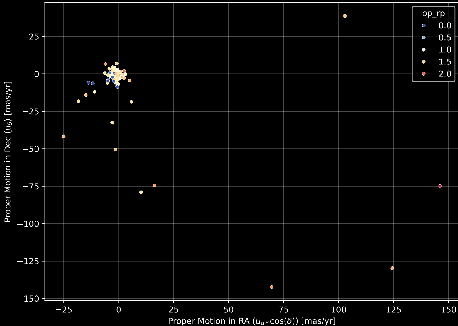
APOGEE DR17 Field: [214+04] Proper Motion Diagram (n= 179)
