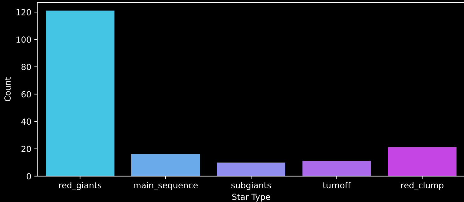
APOGEE DR17 Field: [214+04] Count plot of Star Type
